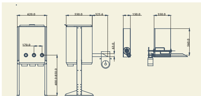
Dimensional sketches
